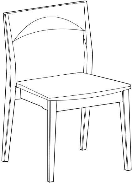
LH-33 upholstered stacking chair • W 500mm (19 11/16") D 521mm (20 9/16") H 762mm (30")
