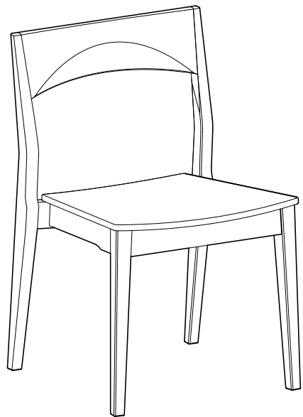
LH-33 ply seat stacking chair • W 500mm (19 11/16") D 519mm (20 7/16") H 762mm (30")
